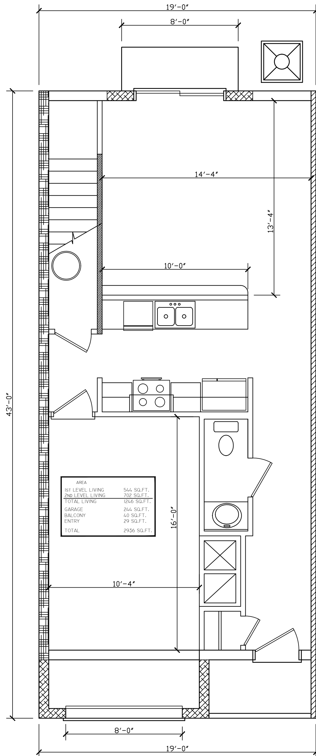
1ST LEVEL FLOOR PLAN
