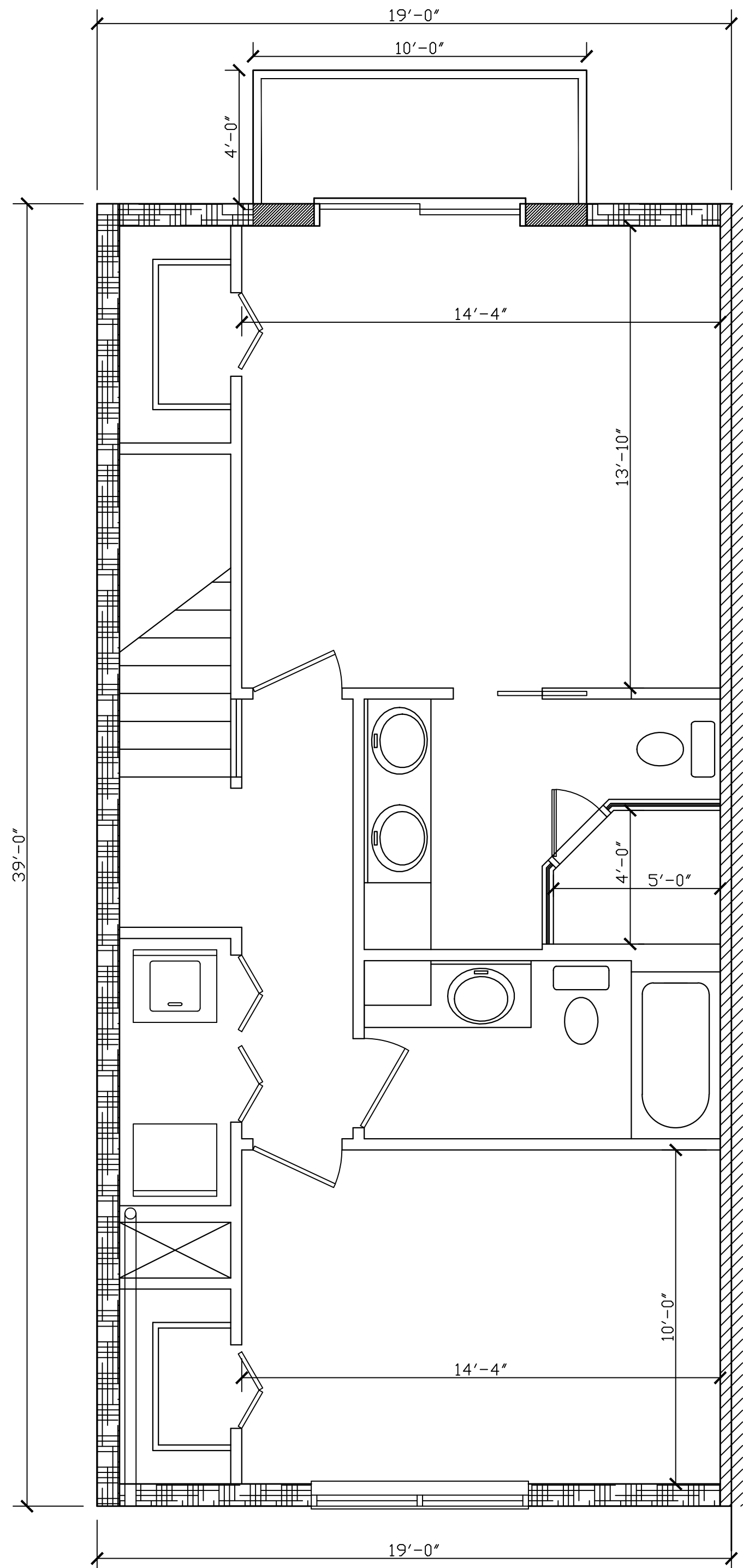
2ND LEVEL FLOOR PLAN
